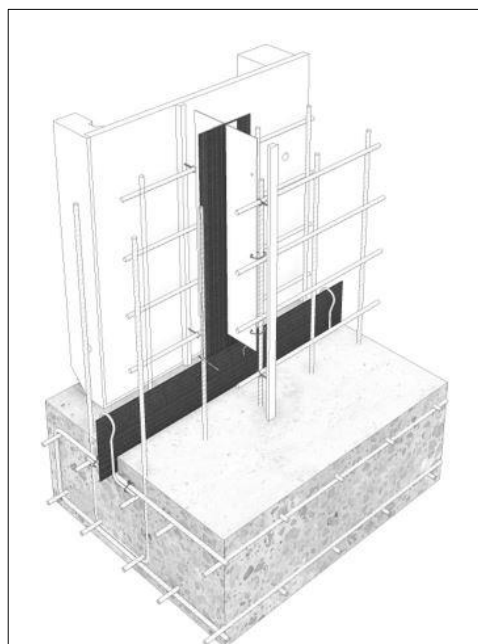
Abb. 3 – Regeldetail 3D
