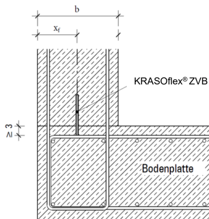
Abb. 2 – Regeldetail 2D
