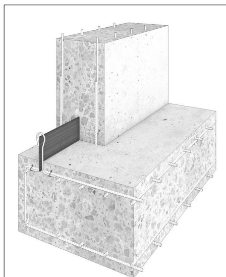
Abb. 1 – Regeldetail 3D
