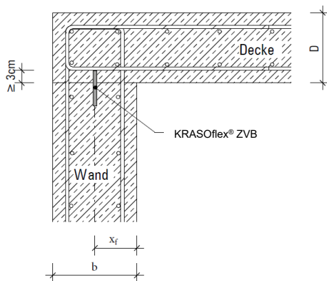
Abb. 10 – Regeldetail 2D
