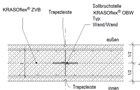
Abb. 4 – Regeldetail 2D
